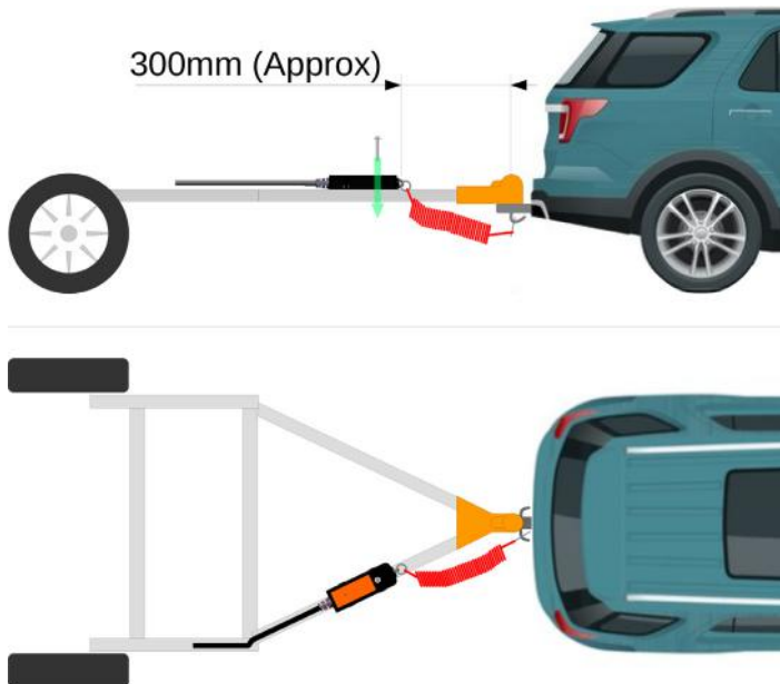
Figure 1: TrailSafe mounting diagram
