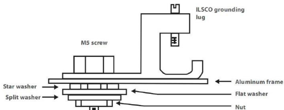
For module with \Phi 5.1 mm grounding holes
