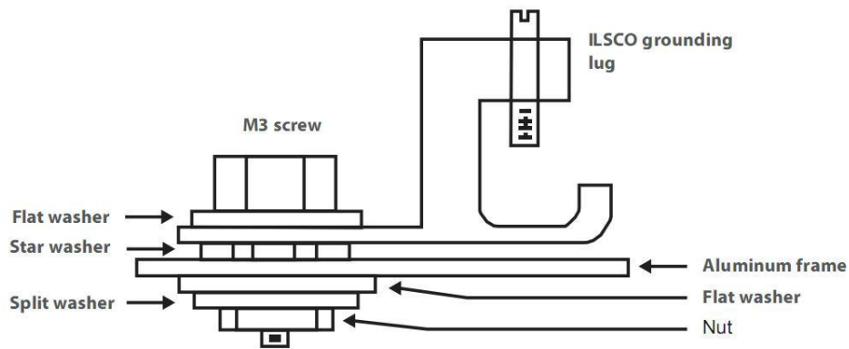
For module with \Phi 4 mm grounding holes
