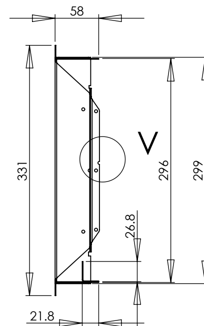
SECTION U-U
