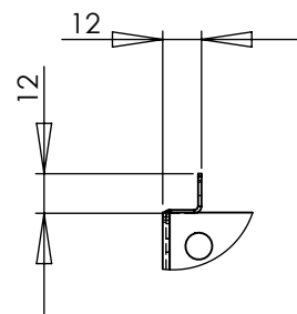
DETAIL U SCALE 2 : 5
